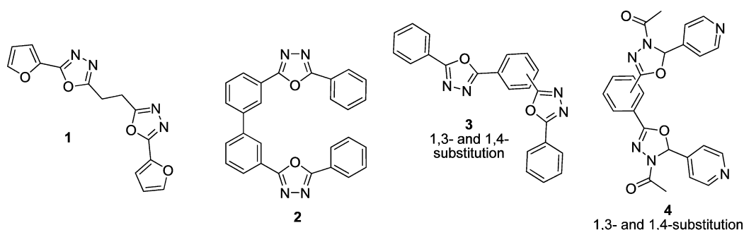
Scheme 1. Examples of Bis-(1,3,4-oxadiazoles) Grafted on Different Aromatic Rings or on the Same Ring As 1,3- or 1,4-Disubstituents
