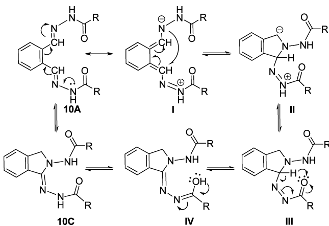
Scheme 6. Proposed Reaction Mechanism for the Transformation 10A to 10C
