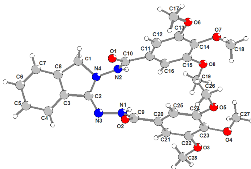
Figure 1. Molecular structure of compound 10Ca-Z , showing the atom numbering scheme. Selected bonds lengths (Å): C2–N4, 1.379(4); C2–N3, 1.287(4); C1–N4, 1.471(4); C1–C8, 1.497(5); N4–N2, 1.390(4); C10–O1, 1.213(4); N1–N3, 1.414(4); C9–O2, 1.245(4).
