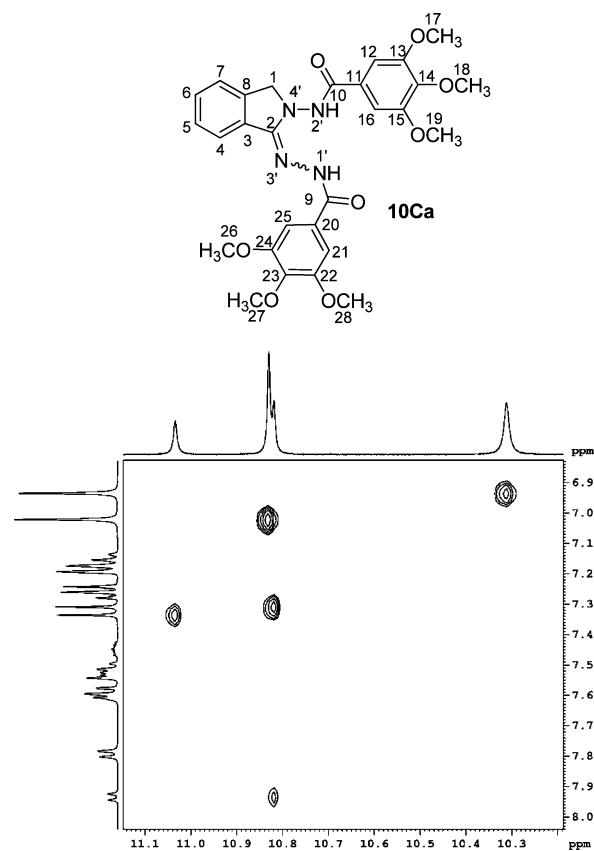
Figure 3. ROESY spectrum (selection) for compound 10Ca in DMSO- d 6 (400 MHz).
