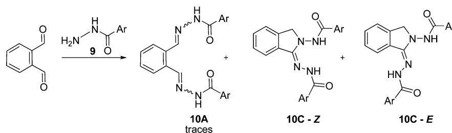
Scheme 4. Structure of the Products Resulted from the Condensation between ortho -Phthalaldehyde and the Aroylhydrazines 9 As Well As the Molar Ratio of Z/E of 10C Determined by 1 H NMR Spectroscopy through Integration of the CH 2 Resonances
