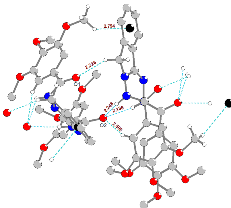
Figure 2. Fragment of the lattice of 10C-Z : a perspective view (along the a axis) reveals the association of molecules through hydrogen bonds and CH– \pi interaction to form supramolecular chain associations. Hydrogen atoms (except the ones involved in different interactions) are omitted for clarity.
