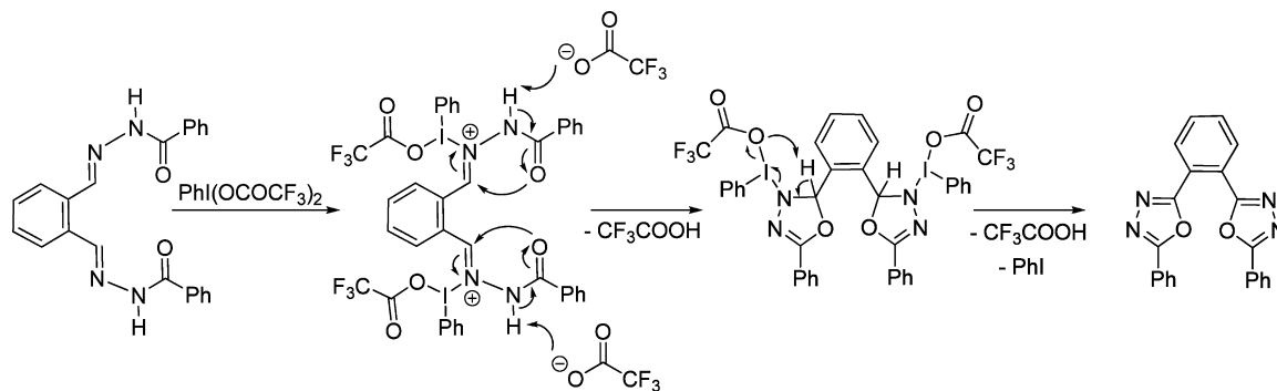
Scheme 5. Proposed Reaction Mechanism for the Oxadiazole Ring Closure
